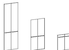
LHD 40-2 790 x 18 x 2206 LMD 40-2 790 x 18 x 1470 LLD 40-2 790 x 18 x 734
