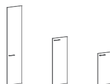
XHD 42-1 422 x 18 x 1900 XMD 42-1 422 x 18 x 1132 XLD 42-1 422 x 18 x 765
