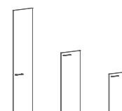
XHD 42-1 422 x 18 x 1900 XMD 42-1 422 x 18 x 1132 XLD 42-1 422 x 18 x 765
