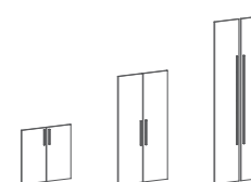
VLD 40-2 790 x 18 x 734 VMD 40-2 790 x 18 x 1470 VHD 40-2 790 x 18 x 2206
