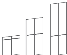
ARLD 40-2 790 x 18 x 734 ARMD 40-2 790 x 18 x 1470 ARHD 40-2 790 x 18 x 2253
