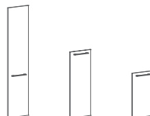
MHD 42-1 422 x 1900 x 18 MMD 42-1 422 x 1132 x 18 MLD 42-1 422 x 765 x 18
